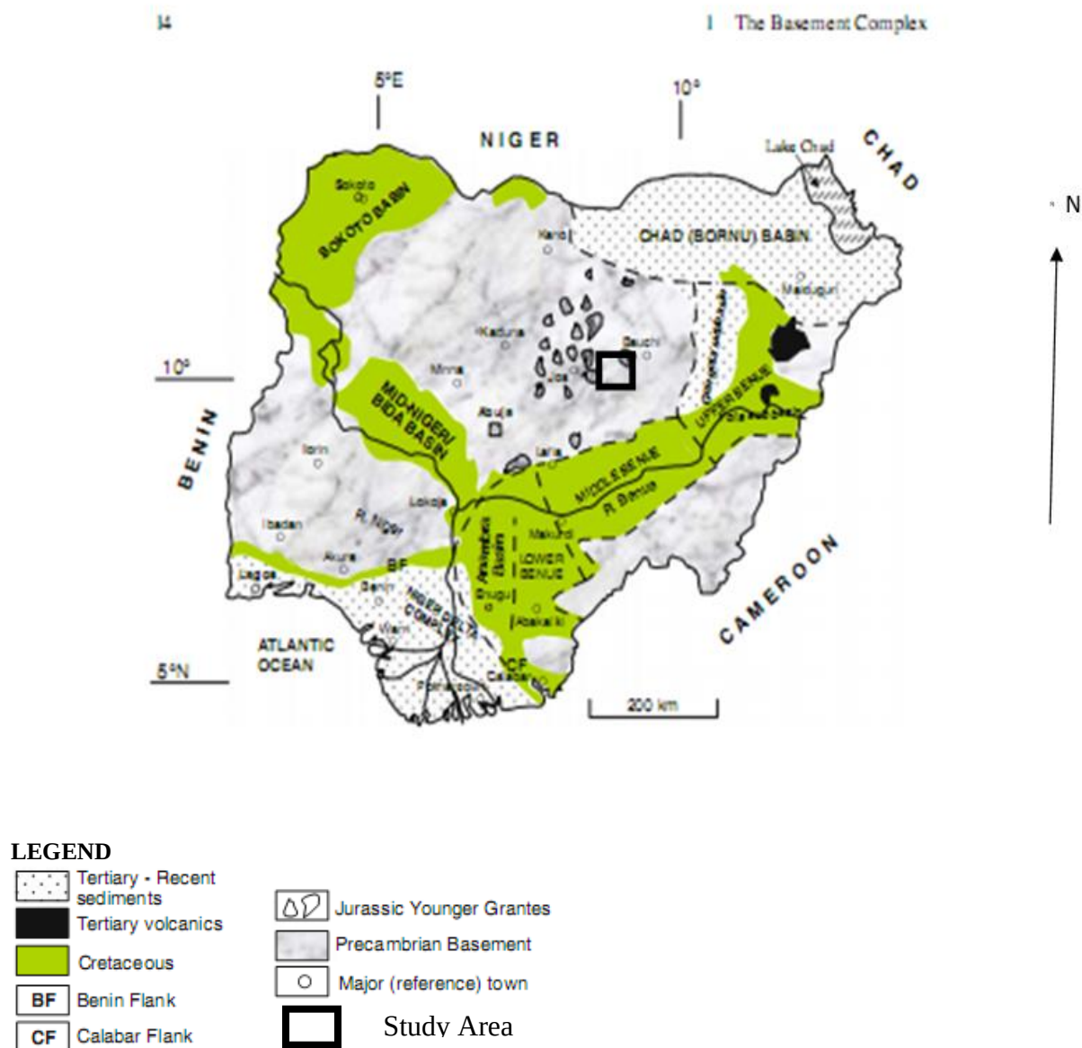
Fig.3. Location Map of the Study Area Modified After Geology
