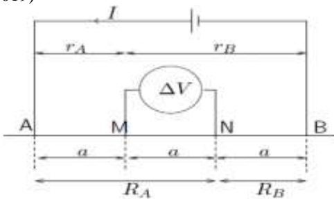
Figure 2: Generalized Four Electrode System. S According to Telford et al. (1990), the geometric factor (K) for Wenner array is given as
